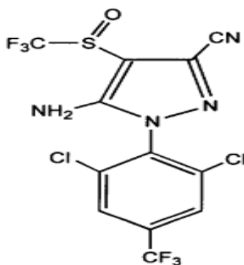
Figure 1. Structural formula of Fipronil.
