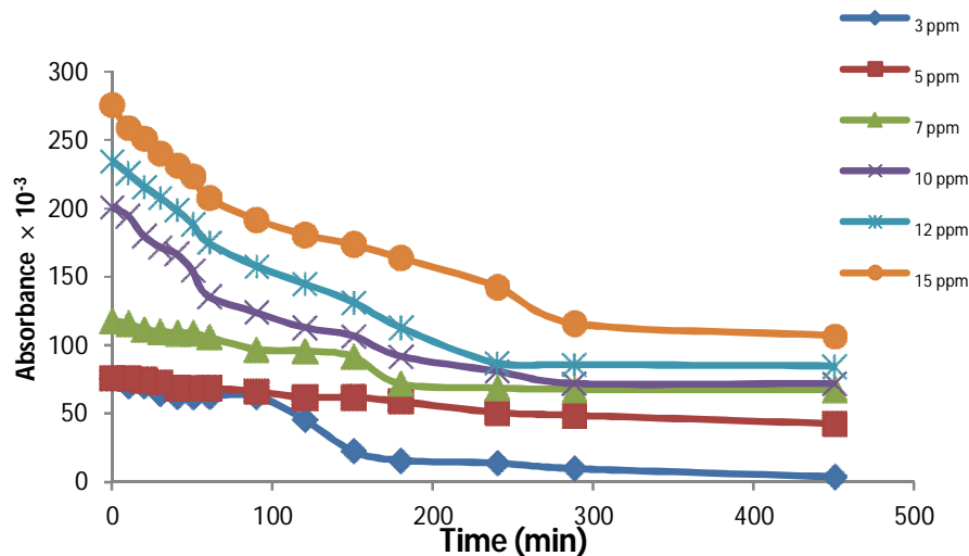
Figure 2. Variation of absorbance with time for Fipronil.
