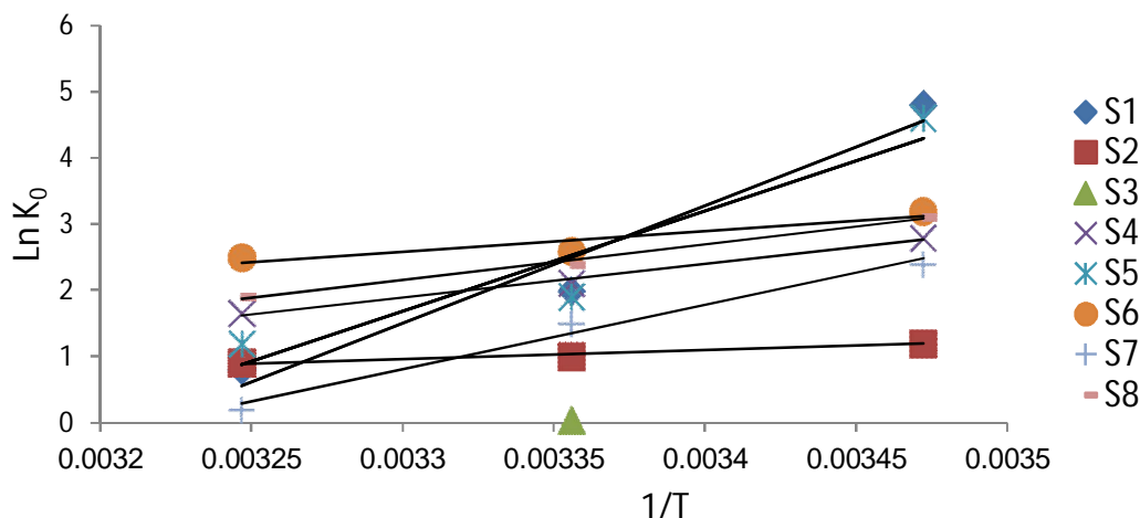
Figure 4. Variation of \ln K_0 with 1/T for adsorption of Fipronil.
