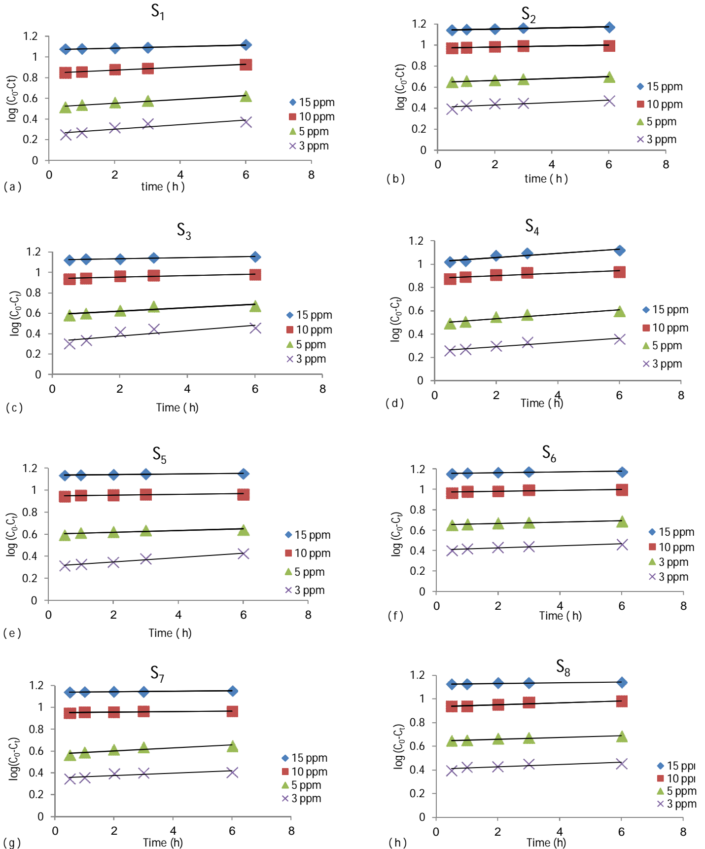
Figure 3. Application of 1 st order rate law for Fipronil on the selected soil samples (a) S 1 , (b) S 2 , (c) S 3 , (d) S 4 , (e) S 5 , (f) S 6 , (g) S 7 , and (h) S 8 .
